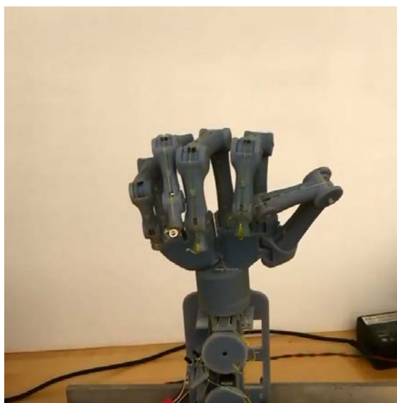
Fig. 5.5. Hand with flexion of each finger
