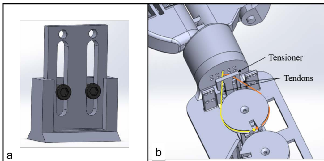
Fig. 4.6. (a) Tensioner, (b) Tendon routing
