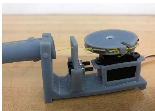
Fig. 5.2. Use of spring in tendon routing
