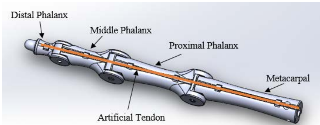
Fig. 4.3. Tendon Route of an Index Finger
